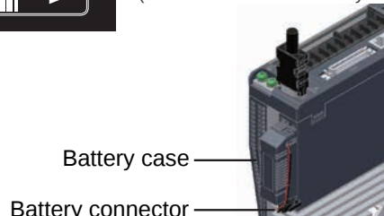
Battery wiring figure
